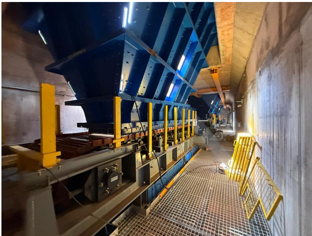
Figure 9: View of inside the reclaim chamber (13 October 2025)
